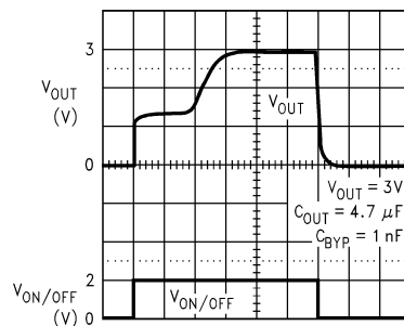
Turn-ON Waveform
