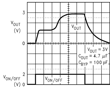
Turn-ON Waveform
