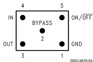
micro SMD, 5 Bump Package (BPA05)
