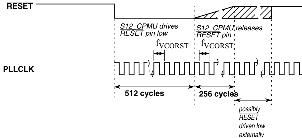
Figure 10-34. RESET Timing
