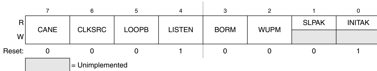
Figure 18-5. MSCAN Control Register 1 (CANCTL1)
