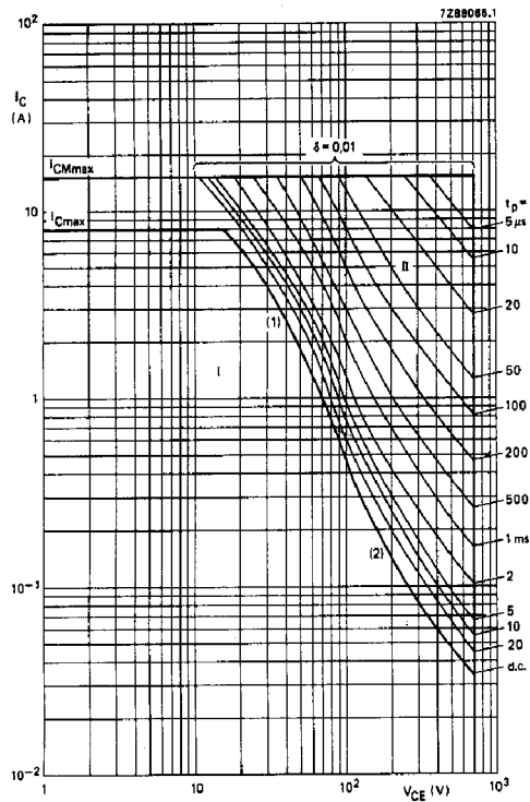
Fig.10. Forward bias safe operating area. T_{hs} < 25^{\circ}\text{C} (1) P_{tot\ max} line. (2) Second-breakdown limits (independent of temperature). I Region of permissible DC operation. II Permissible extension for repetitive pulse operation.
