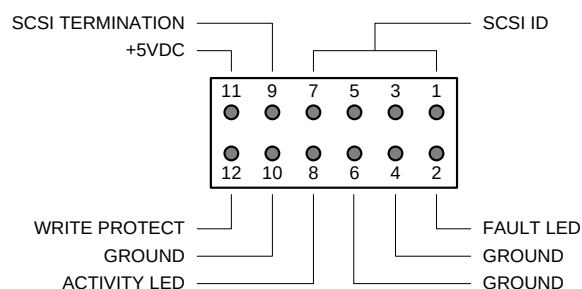
Figure 12: SSD Ultra320 SCSI 3.5" 68-pin Auxiliary Connector Settings
