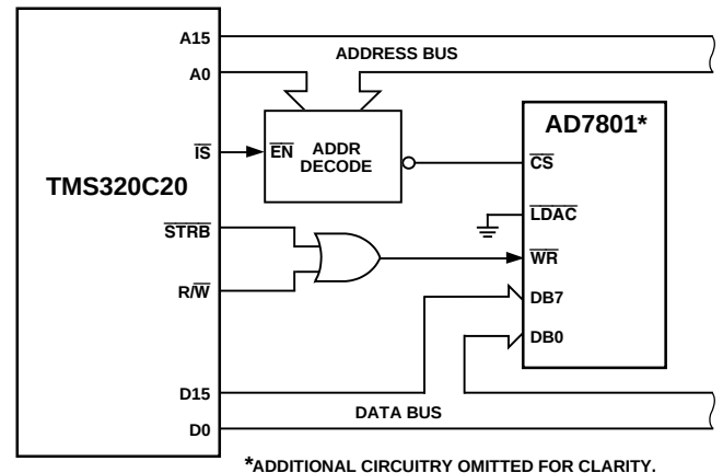
Figure 30. AD7801-TMS320C20 Interface
