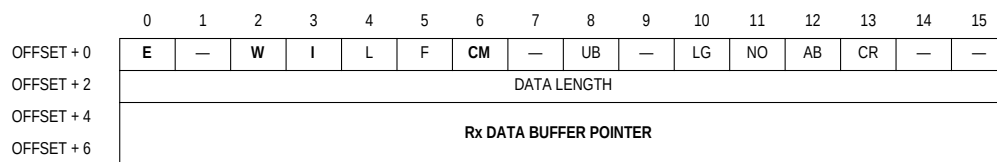
Figure 5-1. Receive Buffer Descriptor (RxBd)
