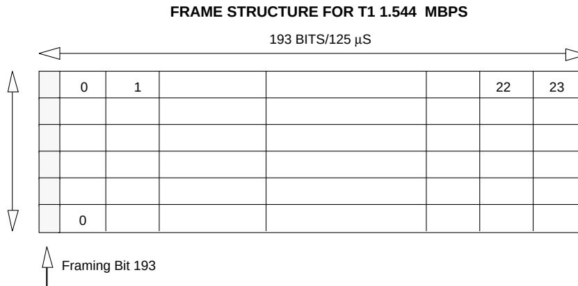
For any station to receive and transmit on a TDM line, it is necessary for it to determine the correct time slot boundary. The service provider or the PTT provides a 4-wire interface with a continuous bit stream coming down the line. The T1 and E1 have information embedded in the data stream that delineates frames. The bit pattern in position 193 in T1 over a period of several frames establishes a synchronization pattern. A station may have the capability to search for this pattern and thus find the correct time for frame synchronization. In a similar way, time slots 0 and 16 are reserved not only for synchronization but also for signaling in the E1 interface.
