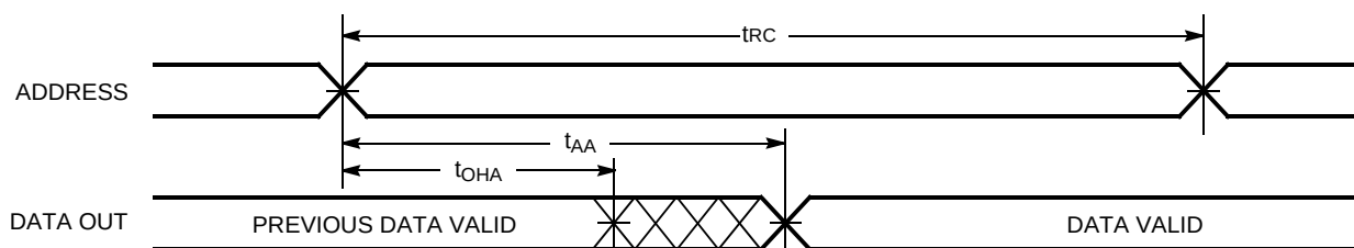
Figure 3. Read Cycle No. 2 ( \overline{\text{OE}} controlled) [10, 16, 17]
