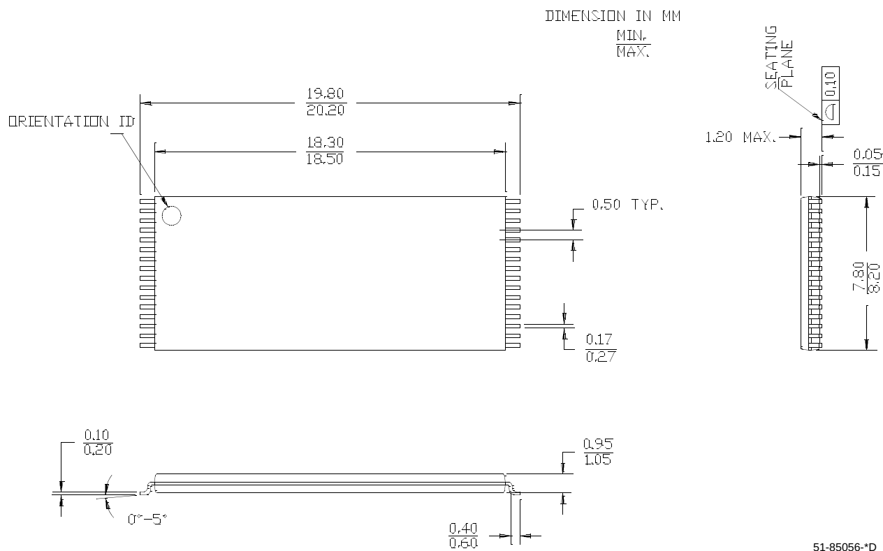
Figure 8. 32-Pin Thin Small Outline Package Type I (8 x 20 mm), 51-85056
