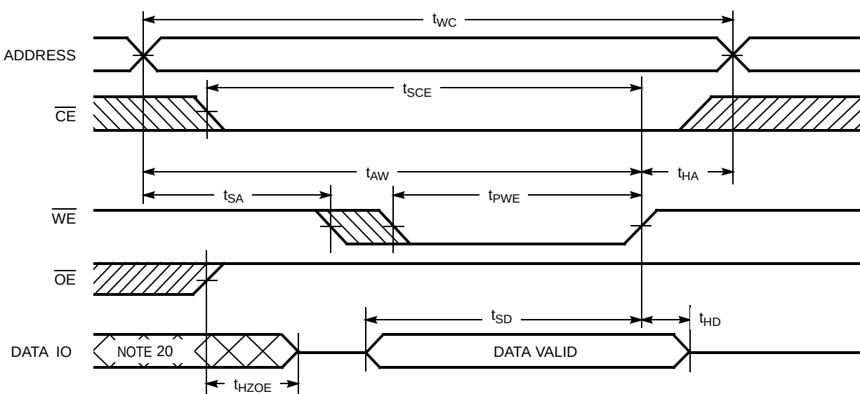
Figure 4. Write Cycle No. 1 ( \overline{\text{WE}} controlled) [10, 15, 18, 19]
