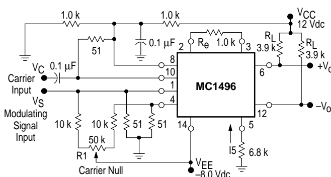
Figure 27. Balanced Modulator-Demodulator
