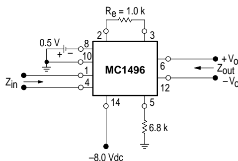
Figure 6. Input-Output Impedance
