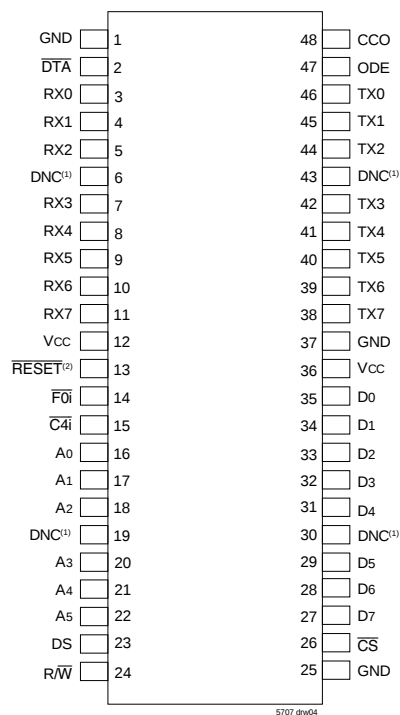
TSSOP: 0.50mm pitch, 12.50mm x 6.10mm (SO48-1, order code: PV) TOP VIEW
