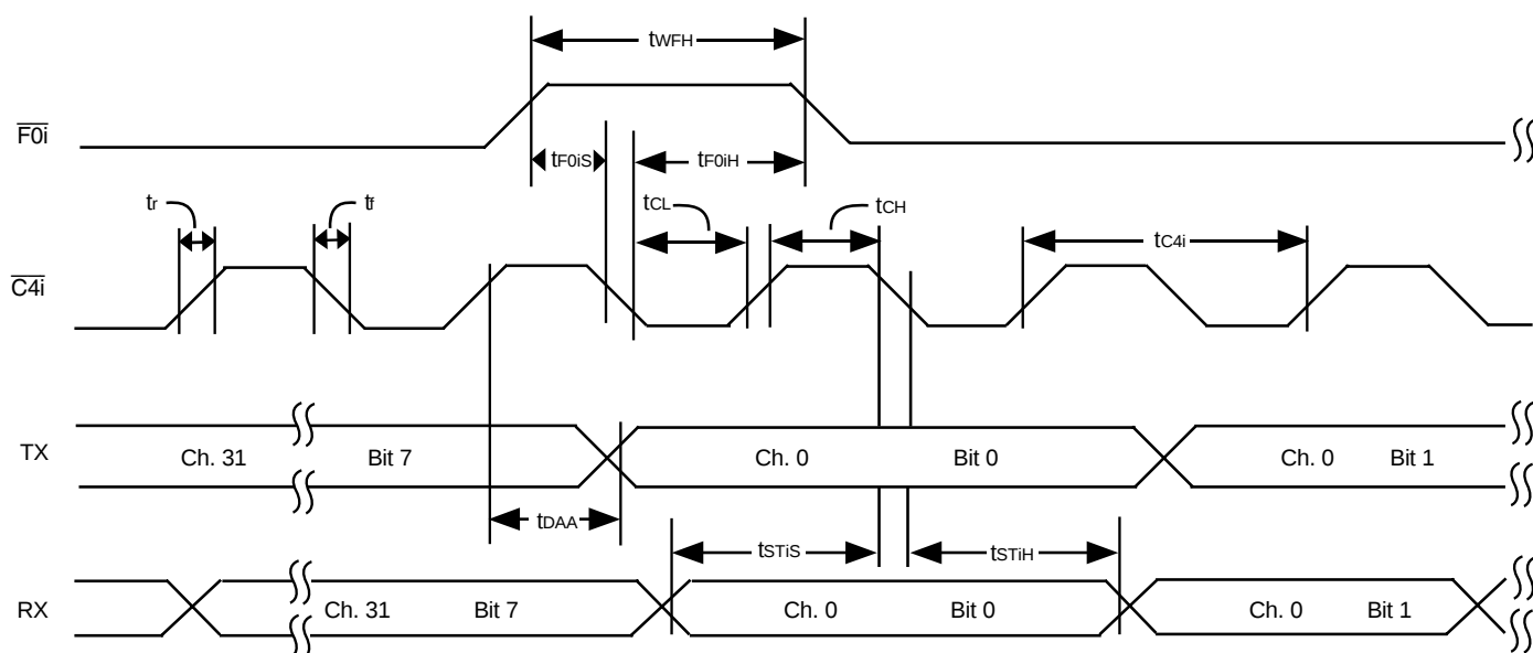
Figure 8. GCI Timing
