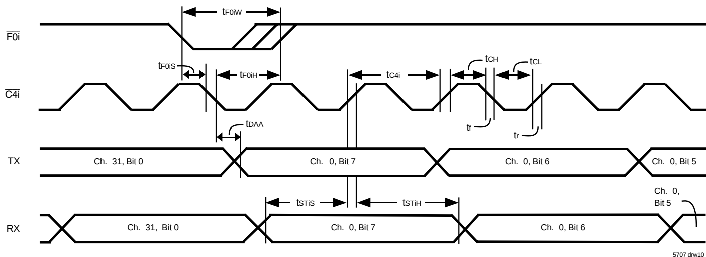
Figure 7. ST-BUS® Timing
