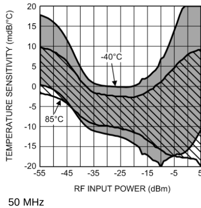
Figure 49. Temperature Sensitivity (Mean \pm 3 Sigma) vs RF Input Power
