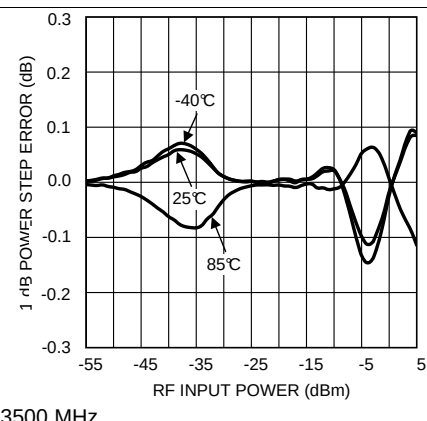
Figure 36. Error For 1-dB Input Power Step vs RF Input Power
