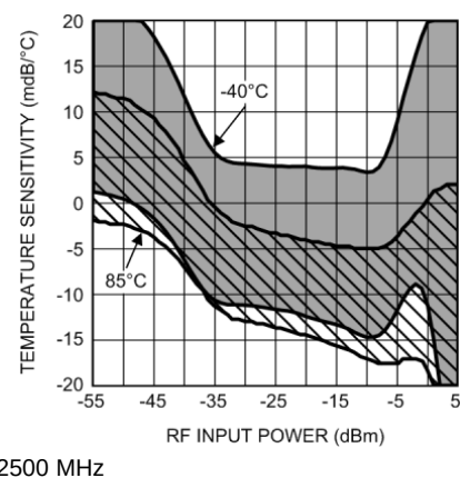
Figure 52. Temperature Sensitivity (Mean \pm 3 Sigma) vs RF Input Power
