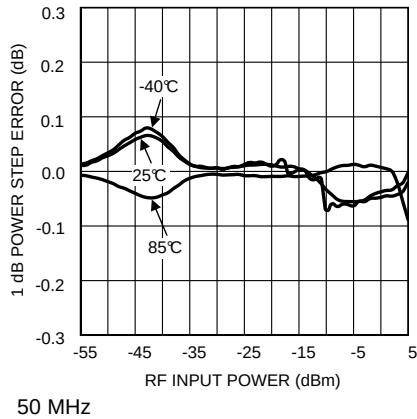
Figure 31. Error For 1-dB Input Power Step vs RF Input Power
