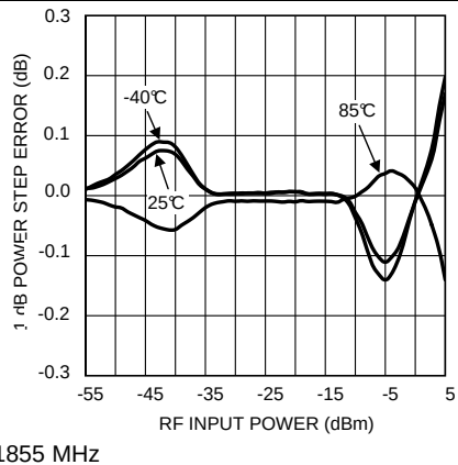
Figure 33. Error For 1-dB Input Power Step vs RF Input Power
