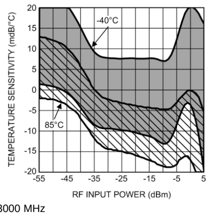
Figure 53. Temperature Sensitivity (Mean \pm 3 Sigma) vs RF Input Power
