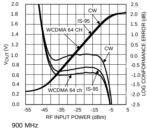
Figure 55. Output Voltage and Log Conformance Error vs RR Input Power for Various Modulation Types
