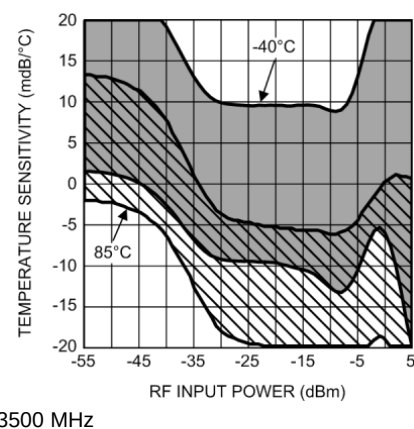
Figure 54. Temperature Sensitivity (Mean \pm 3 Sigma) vs RF Input Power
