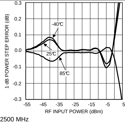
Figure 34. Error For 1-dB Input Power Step vs RF Input Power
