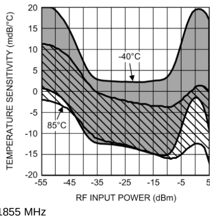
Figure 51. Temperature Sensitivity (Mean \pm 3 Sigma) vs RF Input Power
