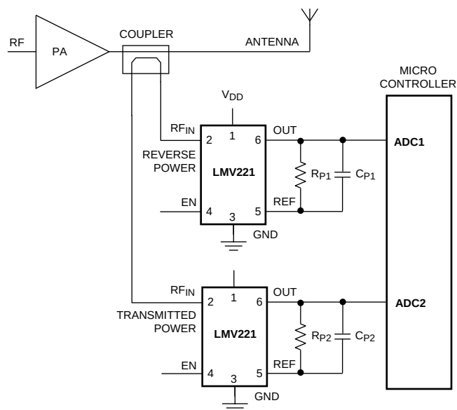
Figure 82. VSWR Application
