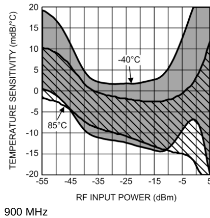
Figure 50. Temperature Sensitivity (Mean \pm 3 Sigma) vs RF Input Power
