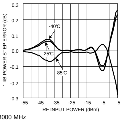
Figure 35. Error For 1-dB Input Power Step vs RF Input Power
