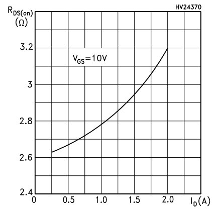
Figure 8. Static drain-source on resistance
