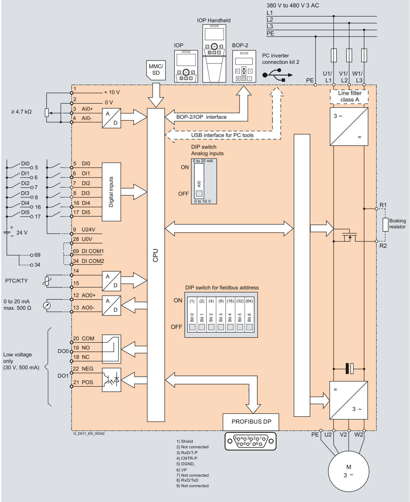
Connection example SINAMICS G120C, PROFIBUS DP version
