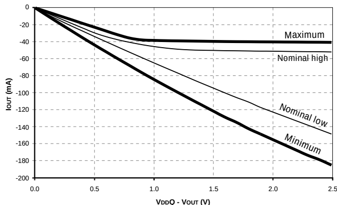
Figure 10: Pull-Up Characteristics
