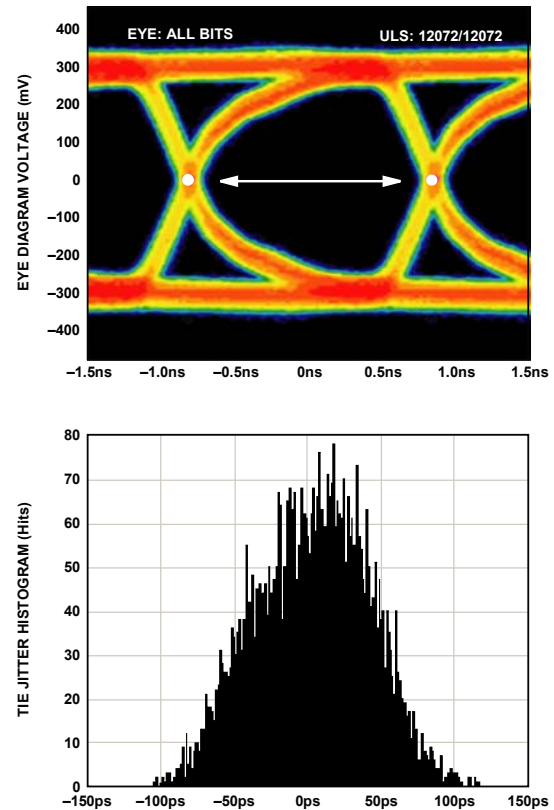
Figure 62. Data Eye for LVDS Outputs in ANSI-644 Mode with 100 \Omega Termination On and Trace Lengths Greater Than 24 Inches on Standard FR-4
