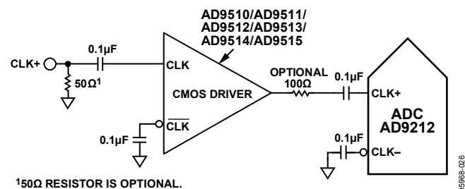
Figure 55. Single-Ended 3.3 V CMOS Sample Clock
