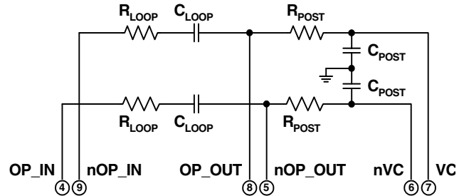
Figure 4: External Loop Filter
