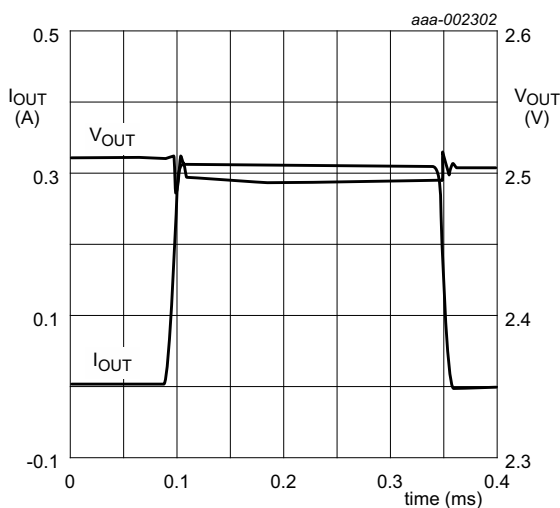
Fig 16. Load regulation for LD6836CX4/25P
