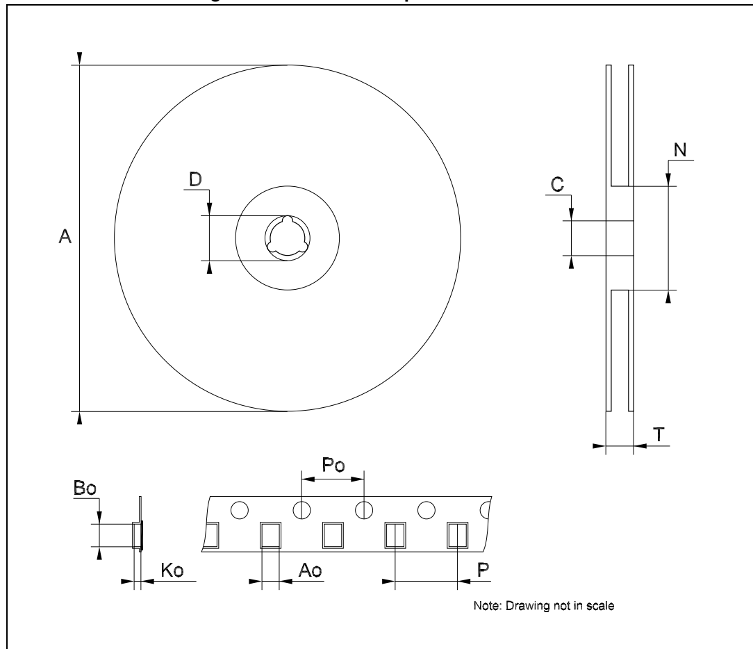
Figure 22. SOT323-5L tape and reel outline
