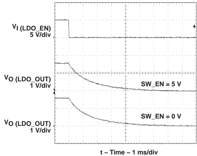
Figure 10. LDO Turnoff Delay and Fall Time With 4.7 \mu\text{F} Load (LDO_OUT Shorted With LDO_PLDN)
