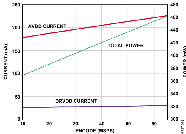
Figure 57. Supply Current vs. f_{\text{SAMPLE}} for f_{\text{IN}} = 10.3 \text{ MHz} , f_{\text{SAMPLE}} = 65 \text{ MSPS}
