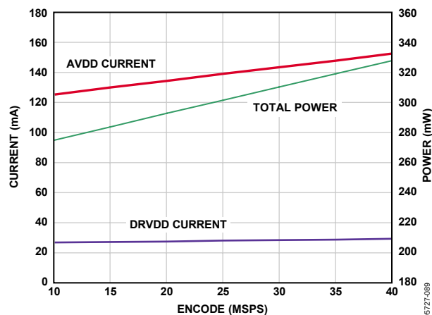
Figure 56. Supply Current vs. f_{\text{SAMPLE}} for f_{\text{IN}} = 10.3 \text{ MHz} , f_{\text{SAMPLE}} = 40 \text{ MSPS}
