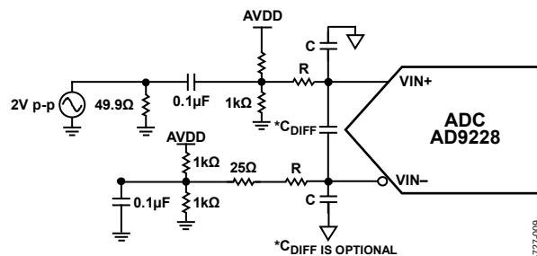
Figure 48. Single-Ended Input Configuration
