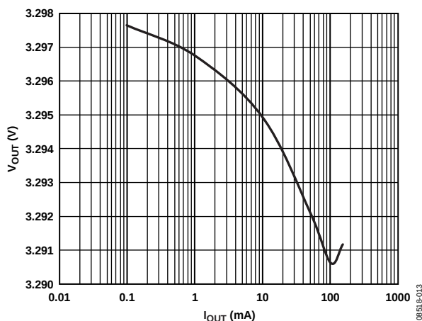
Figure 8. Output Voltage ( V_{OUT} ) vs. Load Current ( I_{OUT} ) at V_{IN} = 3.7\text{ V} , V_{OUT} = 3.3\text{ V} , T_A = 25^\circ\text{C}
