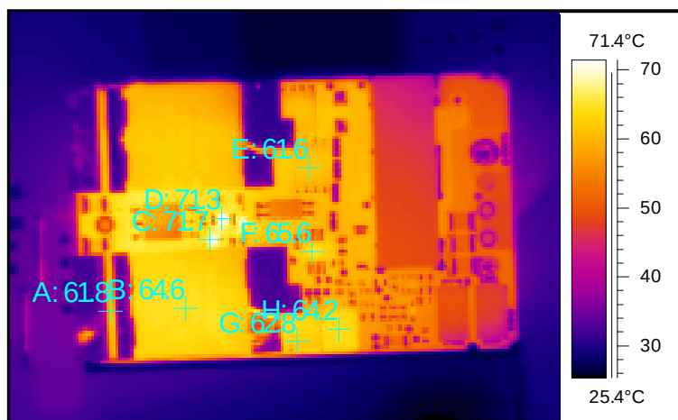
Figure 20 Parallel Airflow at 300 LFM, from output to input (right to left). Ambient Temperature 25 °C. Vin = 48 V, and load current of 12 amps.
