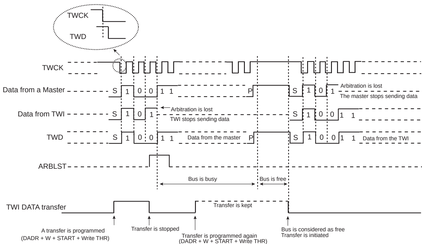
Figure 32-29. Arbitration Cases
