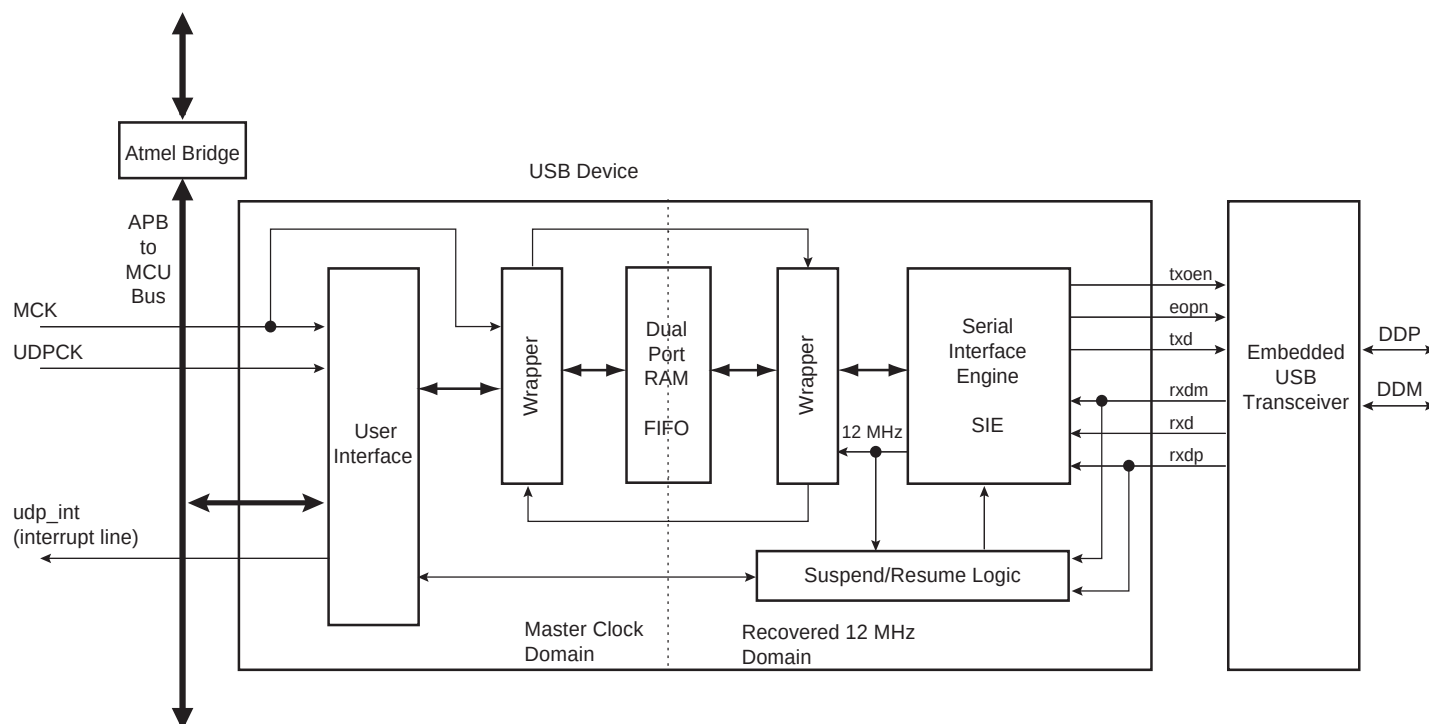
Figure 37-1. Block Diagram
