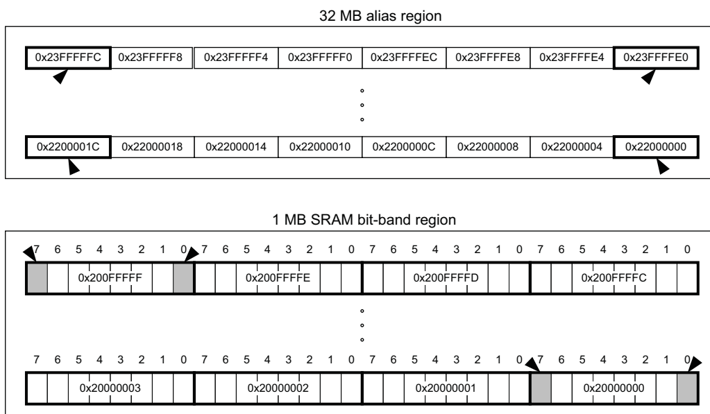
Figure 13-4. Bit-band Mapping
