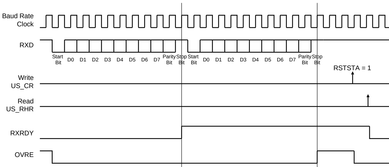
Figure 30-10. Receiver Status
