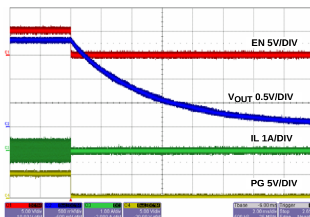
FIGURE 27. SOFT-DISCHARGE SHUTDOWN
