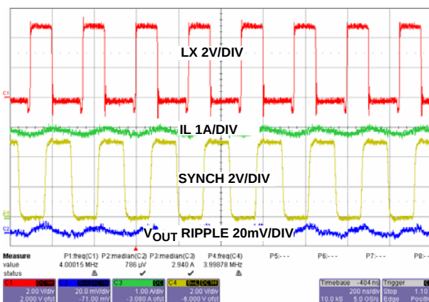
FIGURE 31. STEADY STATE OPERATION AT FULL LOAD (PWM) WITH FREQUENCY = 4MHz
