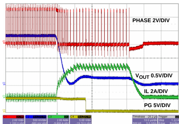
FIGURE 32. OUTPUT SHORT-CIRCUIT
