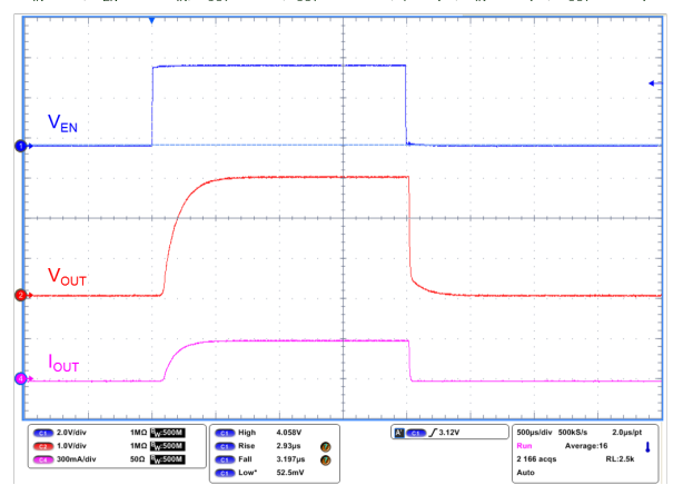
Figure 25. Enable transient
