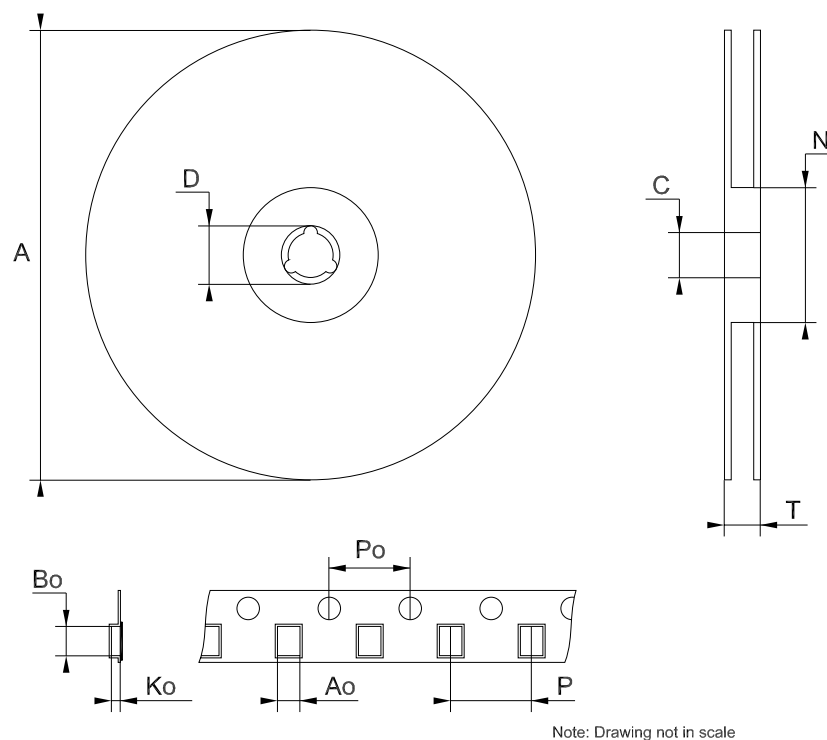
Figure 28. SOT23-5L tape and reel drawing
