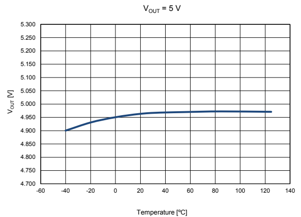
Figure 9. Output voltage vs. temperature ( I_{OUT} = 300 mA )
