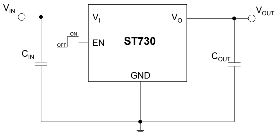
Figure 4. Typical application circuit, fixed version
