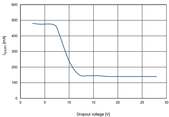
Figure 18. Short circuit current vs. dropout voltage
