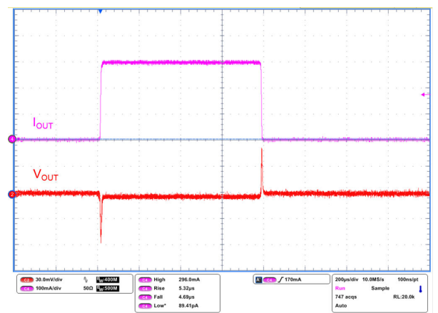
Figure 25. Enable transient
