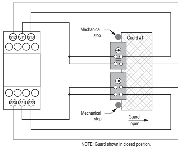
Figure 3. Wiring to two positive-opening safety interlock switches
