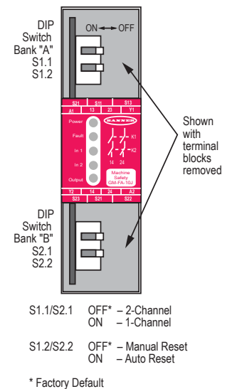
Figure 8. DIP switch configuration settings for reset mode and 1- or 2-channel operation
