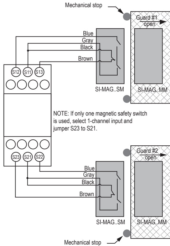
Figure 2. Wiring to two 4-wire coded magnetic safety switches
