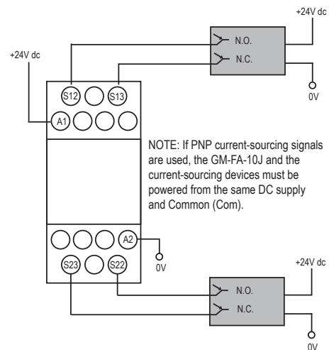
Figure 4. Wiring to two complementary current-sourcing PNP devices
