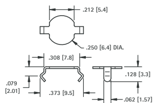
Mounting Detail
