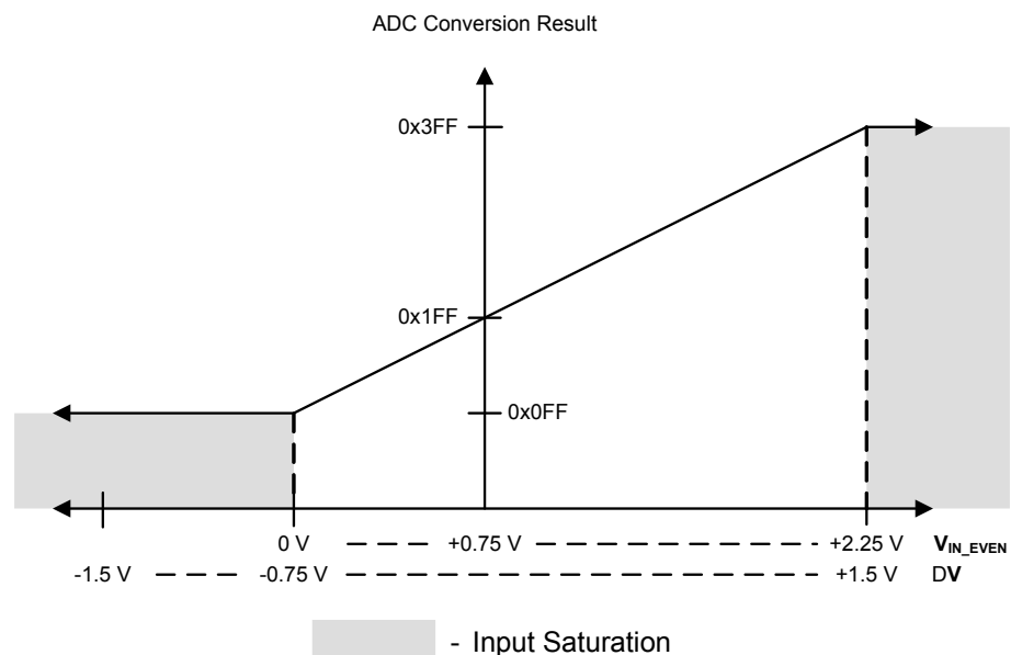
Figure 13-3. Differential Sampling Range, V_{IN\_ODD} = 0.75\text{ V}
