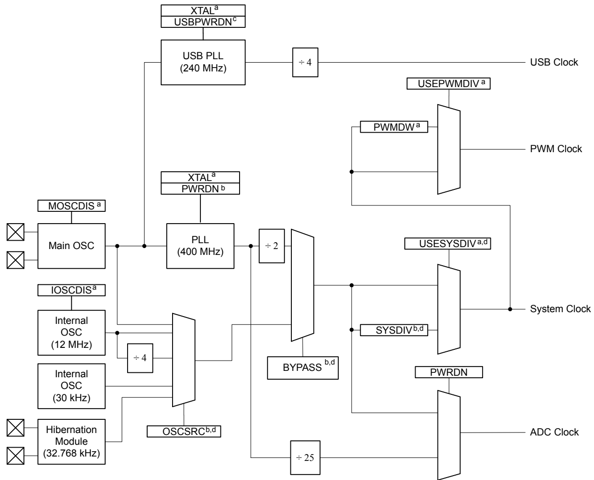
Figure 6-4. Main Clock Tree
