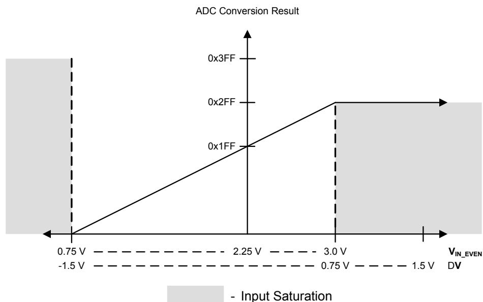
Figure 13-4. Differential Sampling Range, V_{IN\_ODD} = 2.25\text{ V}
