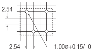
Recommended Footprint Details
