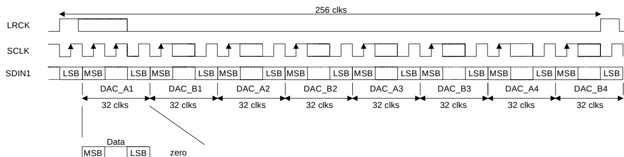
Figure 19. Format 12 - TDM Mode
