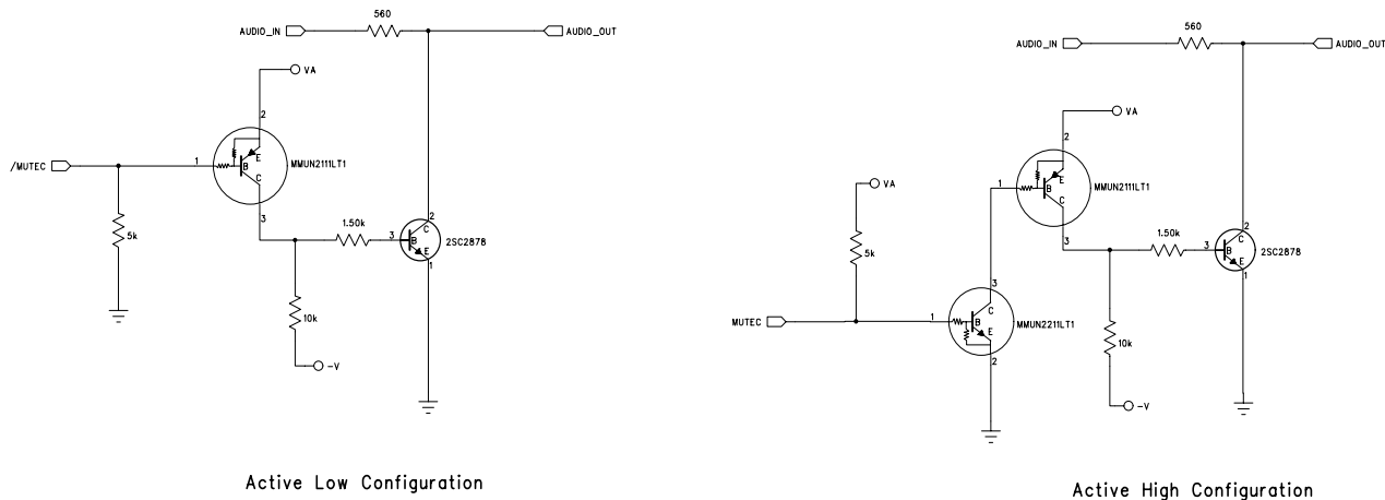
Figure 25. Recommended Mute Circuitry
