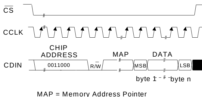
Figure 27. Control Port Timing, SPI Mode
