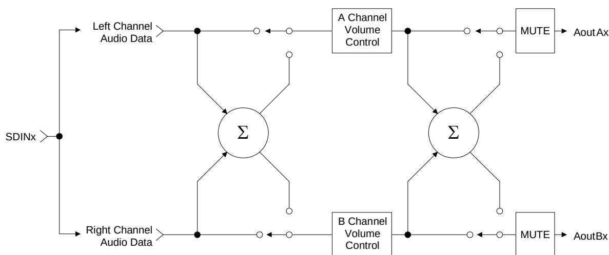
Figure 21. ATAPI Block Diagram (x = channel pair 1, 2, 3, or 4)
