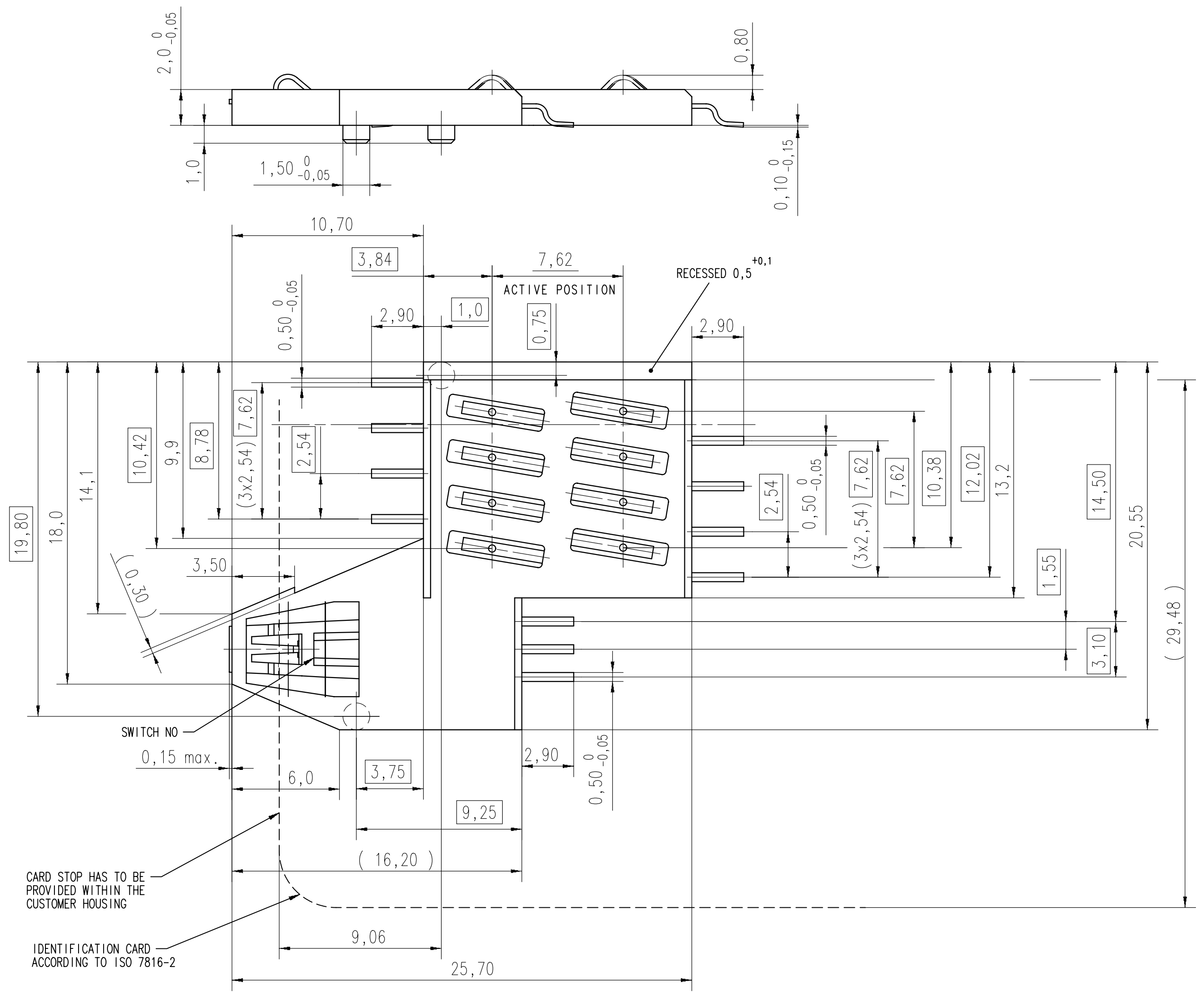
PCB - LAYOUT
