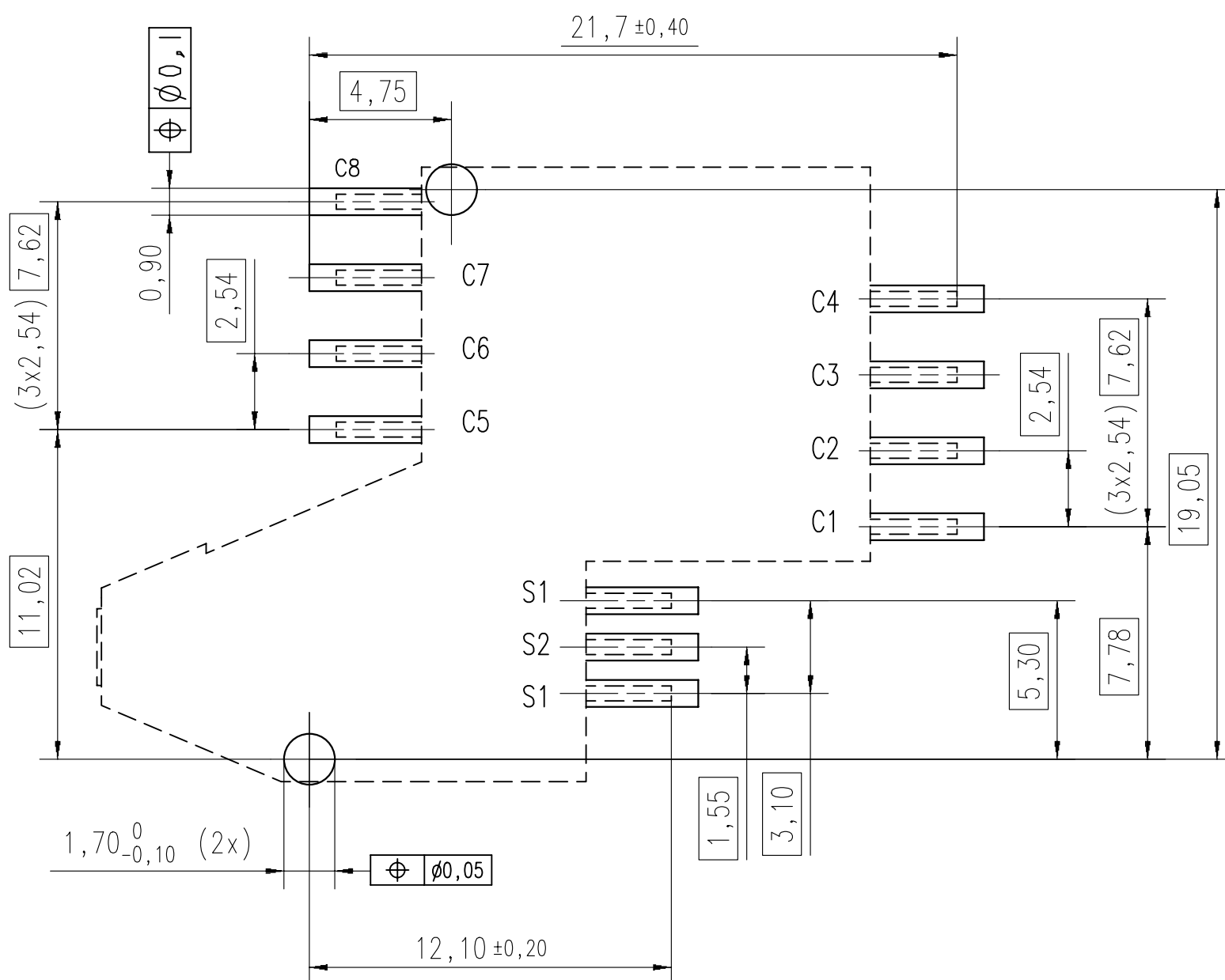
PCB - LAYOUT
