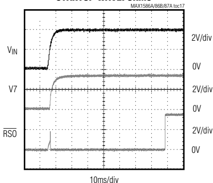
V7 AND \overline{RSO} STARTUP WAVEFORMS
