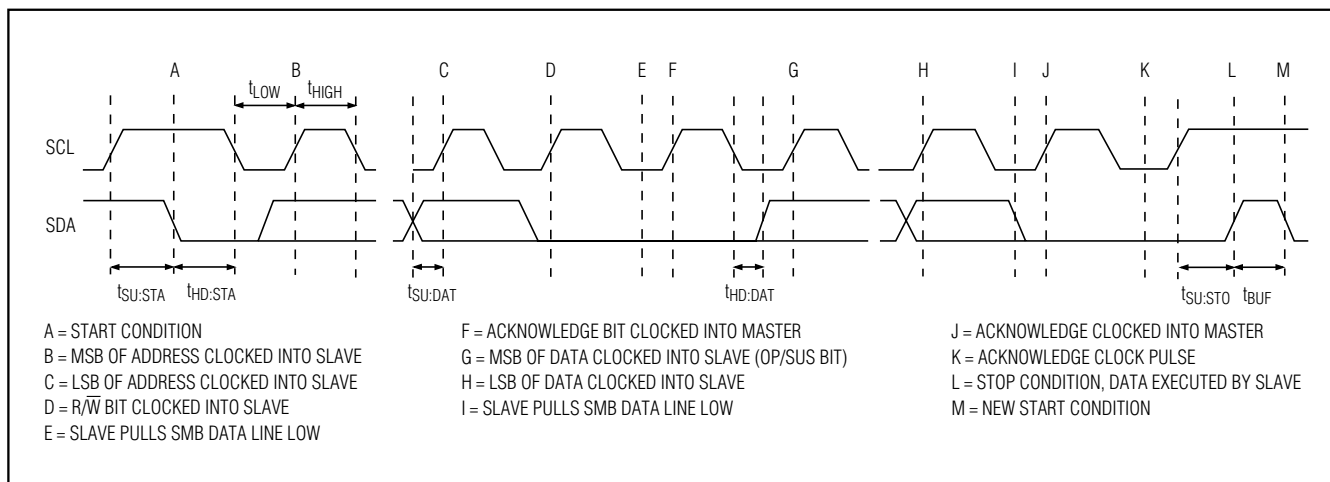
Figure 5. I^2C -Compatible Serial-Interface Timing Diagram
