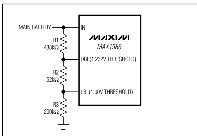
Figure 3. Setting the Low-Battery and Dead-Battery Thresholds with One Resistor Chain. The values shown set a \overline{DBI} threshold of 3.3V and an \overline{LBI} threshold of 3.5V (no resistors are needed for the factory preset thresholds).
