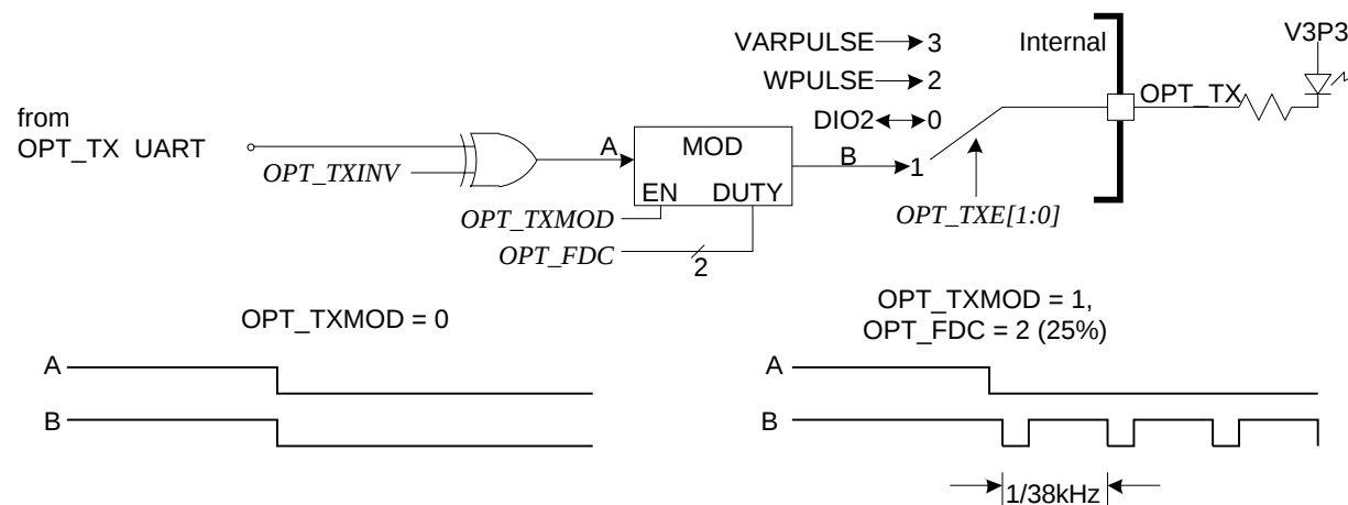
Figure 18: Optical Interface
