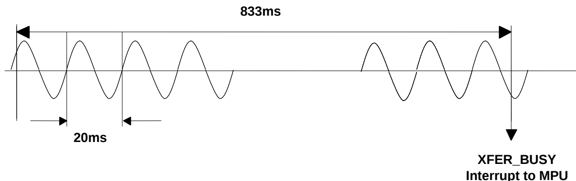
Figure 13: Accumulation Interval
