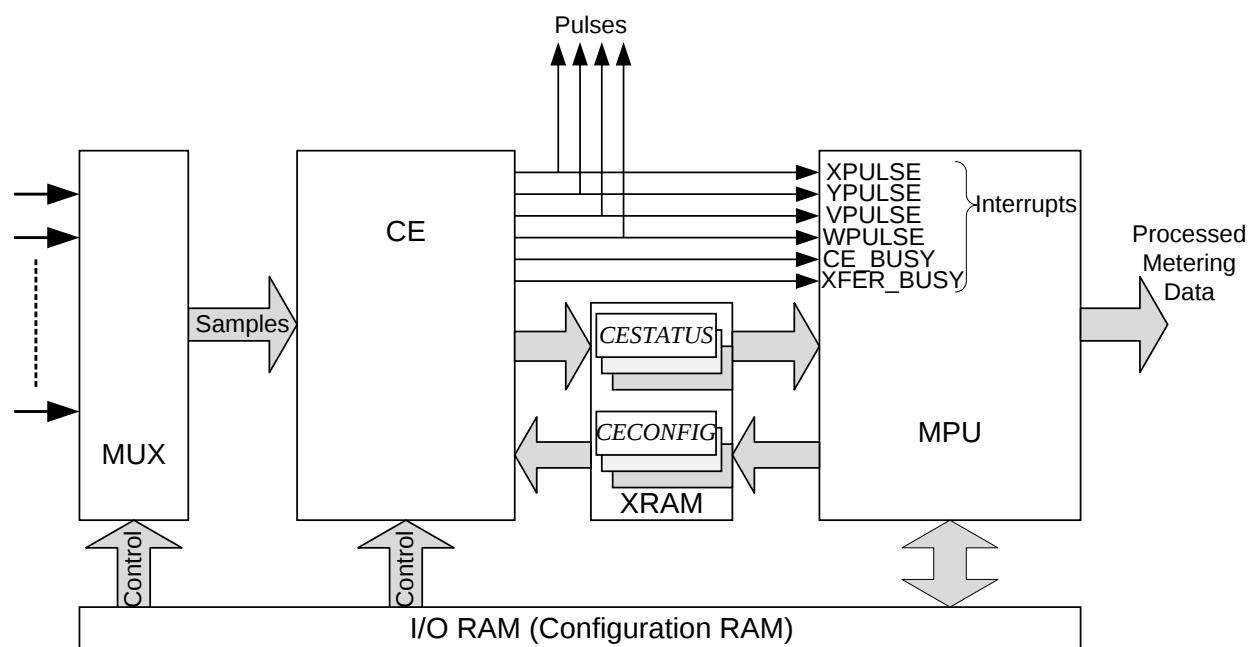
Figure 30: MPU/CE Data Flow
