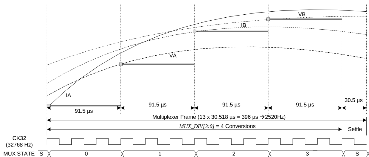
Figure 15: Samples from Multiplexer Cycle ( MUX\_DIV[3:0] = 4 )
