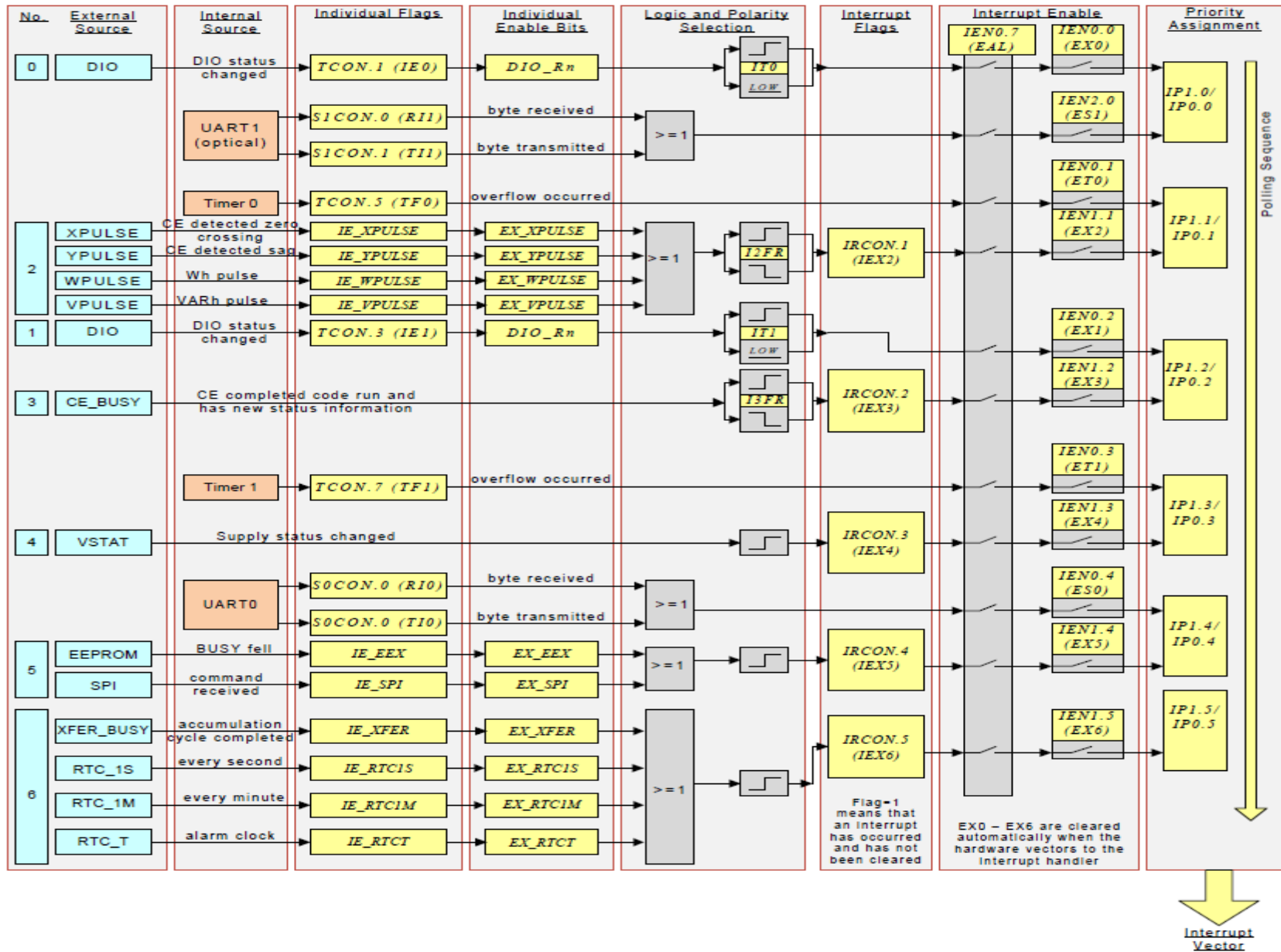
Figure 16: Interrupt Structure
