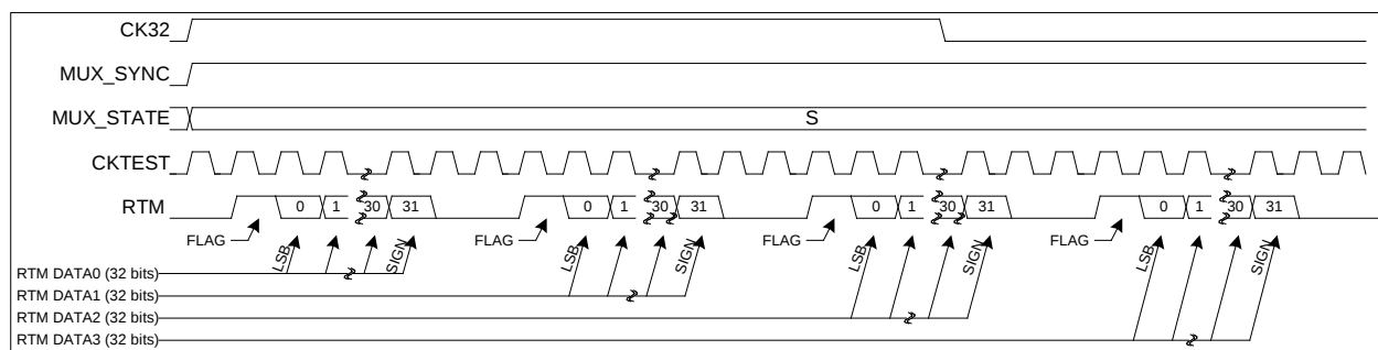
Figure 10: RTM Timing
