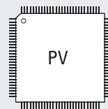
112-Lead LQFP
