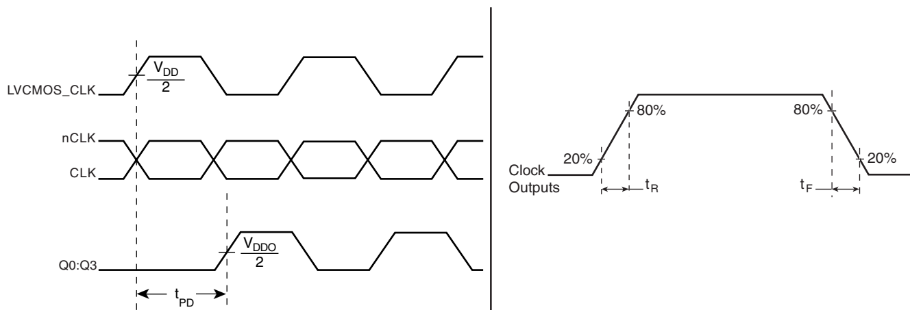
PROPAGATION DELAY
