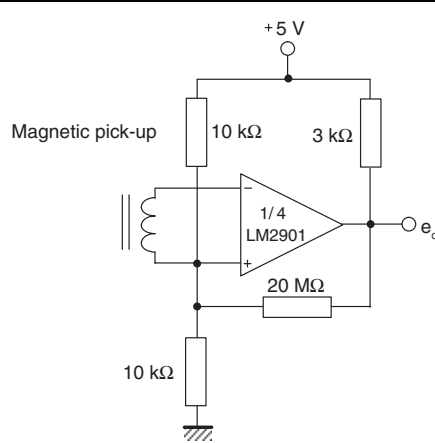
Figure 13. Transducer amplifier
