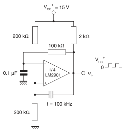
Figure 18. Crystal controlled oscillator
