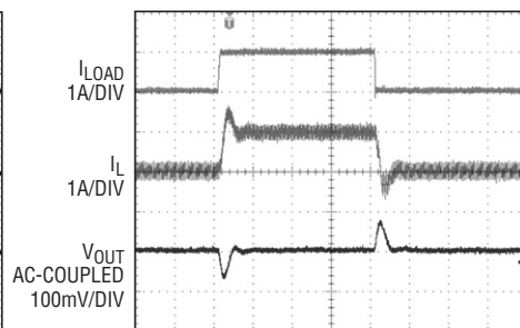
Load Step, Forced Continuous Operation
