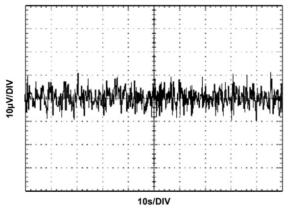
FIGURE 82. V_{OUT} NOISE
