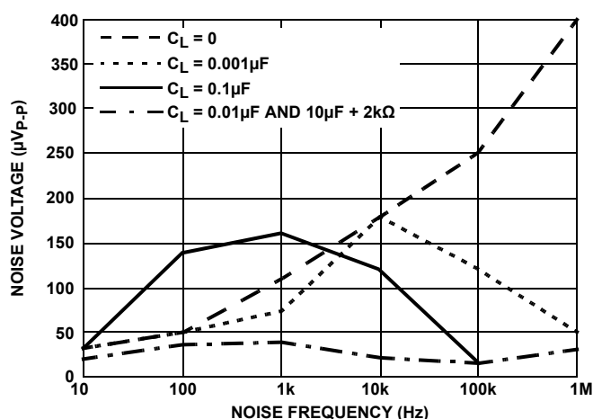
FIGURE 117. NOISE REDUCTION
