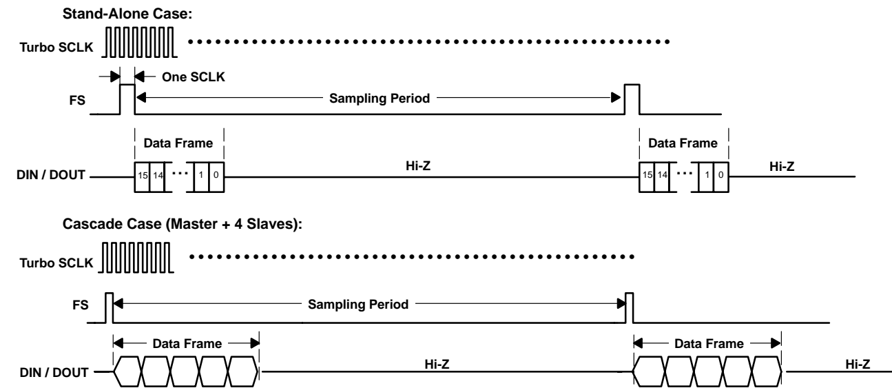
Figure 3–18. Timing Diagram for Turbo Operation
