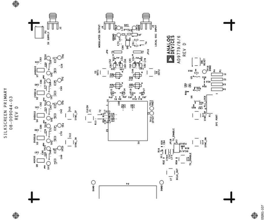
Figure 108. Evaluation Board, Rev. D, Top Silk Screen
