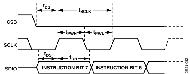
Figure 52. Timing Diagram for SPI Register Write
