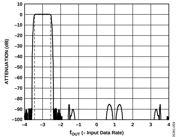
Figure 59. Interpolation/Modulation Combination of -3f_{DAC}/8 Filter
