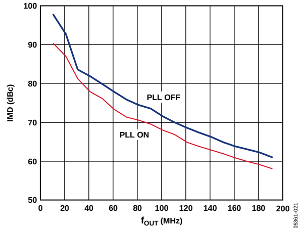
Figure 21. AD9779 Third Order IMD vs. f_{OUT} , 4x Interpolation, f_{DATA} = 100 MSPS, PLL On vs. PLL Off
