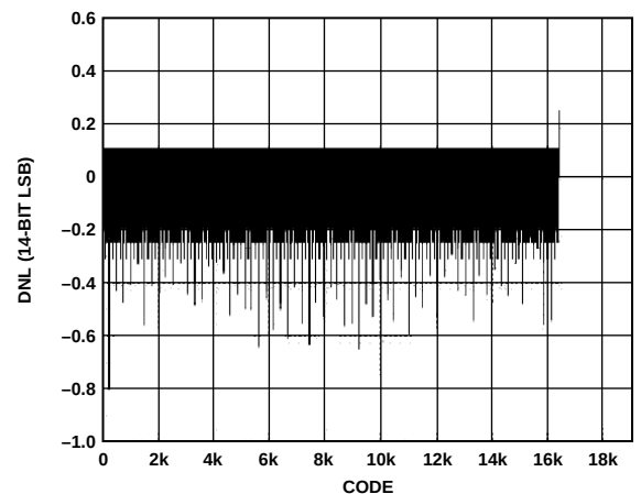
Figure 34. AD9778 Typical DNL
