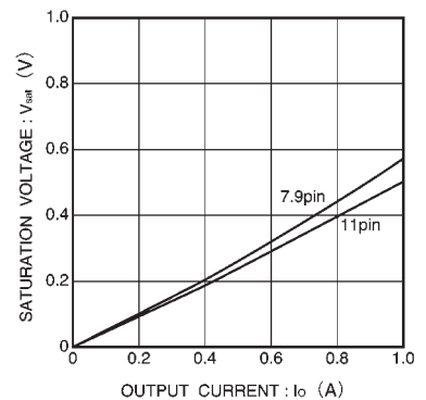
Fig.22 Output saturation voltage vs. output current
