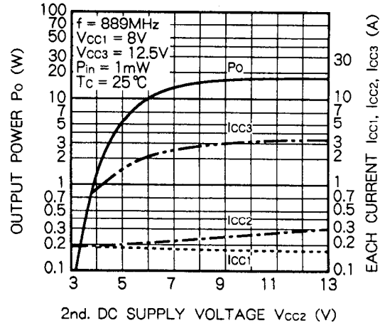
OUTPUT POWER, EACH CURRENT VS. 2nd. DC SUPPLY VOLTAGE CHARACTERISTICS
