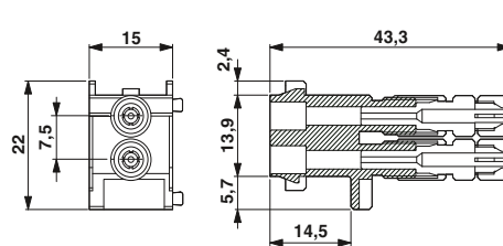
Dimensional drawing: VC-AFOS 2
