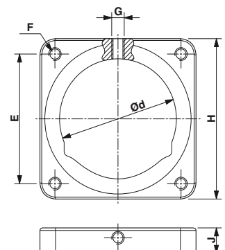
Flange dimensions
