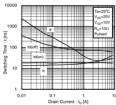
Fig.8 Switching Characteristics
