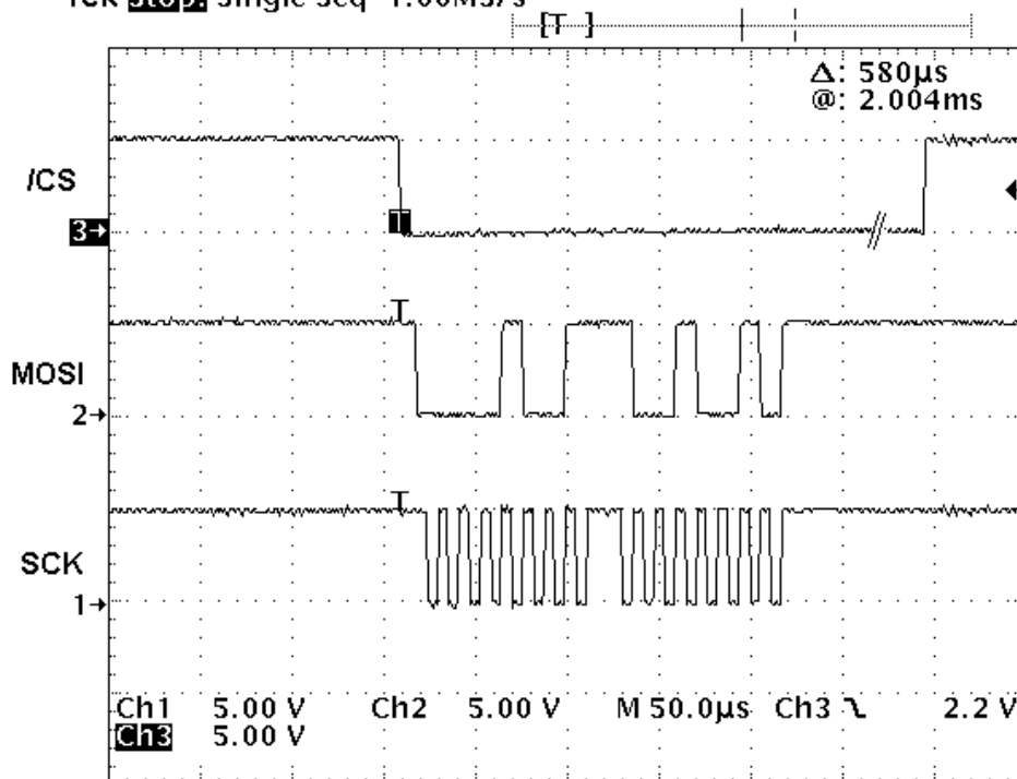
Figure 11: Scope Diagram. Value: 0000100110010010 bin / 0992 hex / 2450 dec ==&gt; 19.14 l/min
