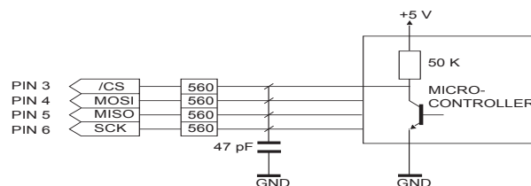
Figure 8: Internal CMOSens ® MFM SPI hardware.
