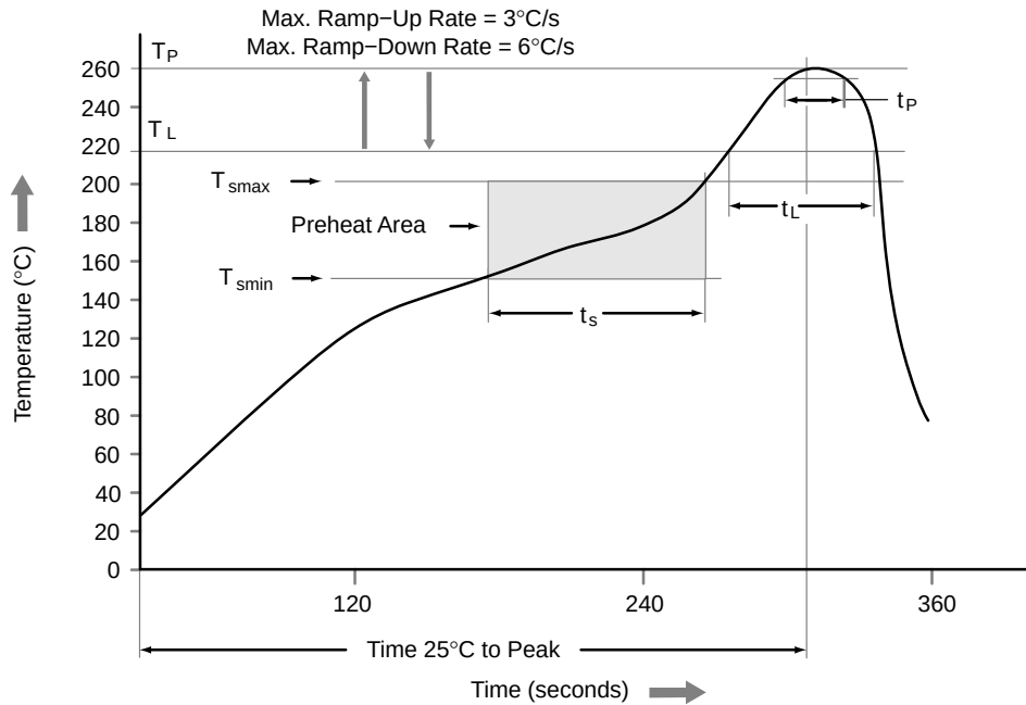
Figure 59. Reflow Profile
