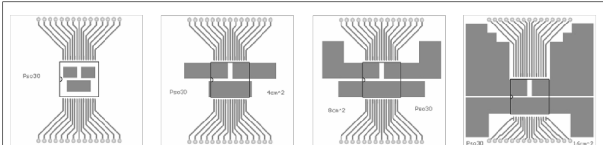
Figure 16. MultiPowerSO-30™ PC board
