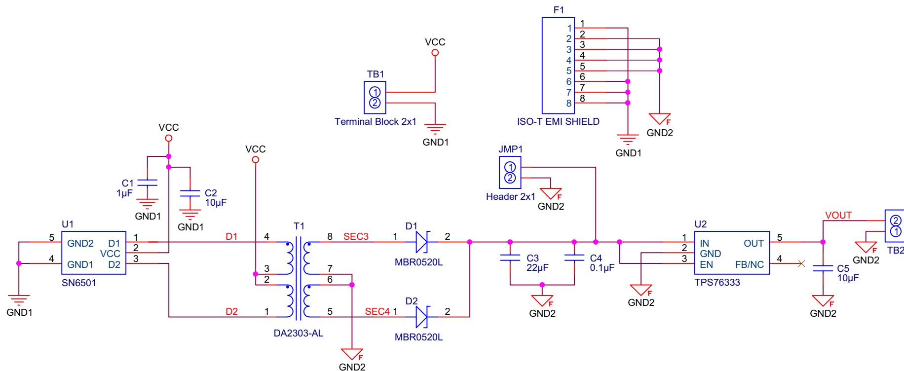
Figure 2. SN6501-3EVM Schematic
