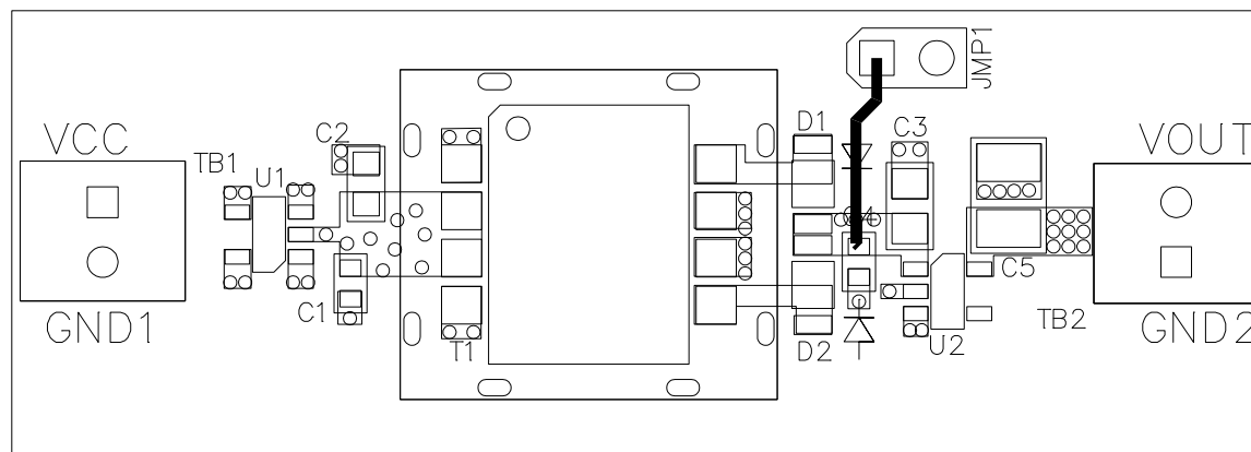
Figure 3. SN6501-3EVM Top Layer View
