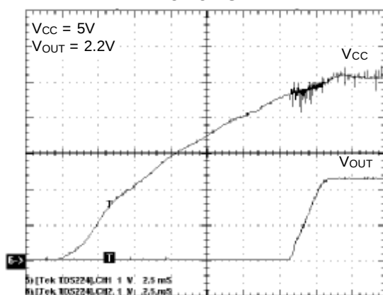
Power On
