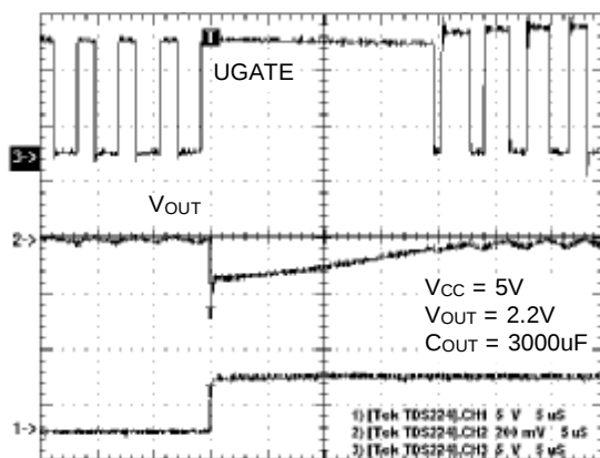
Load Transient
