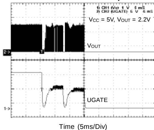
Short Circuit Hiccup
