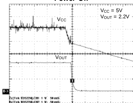
Power Off
