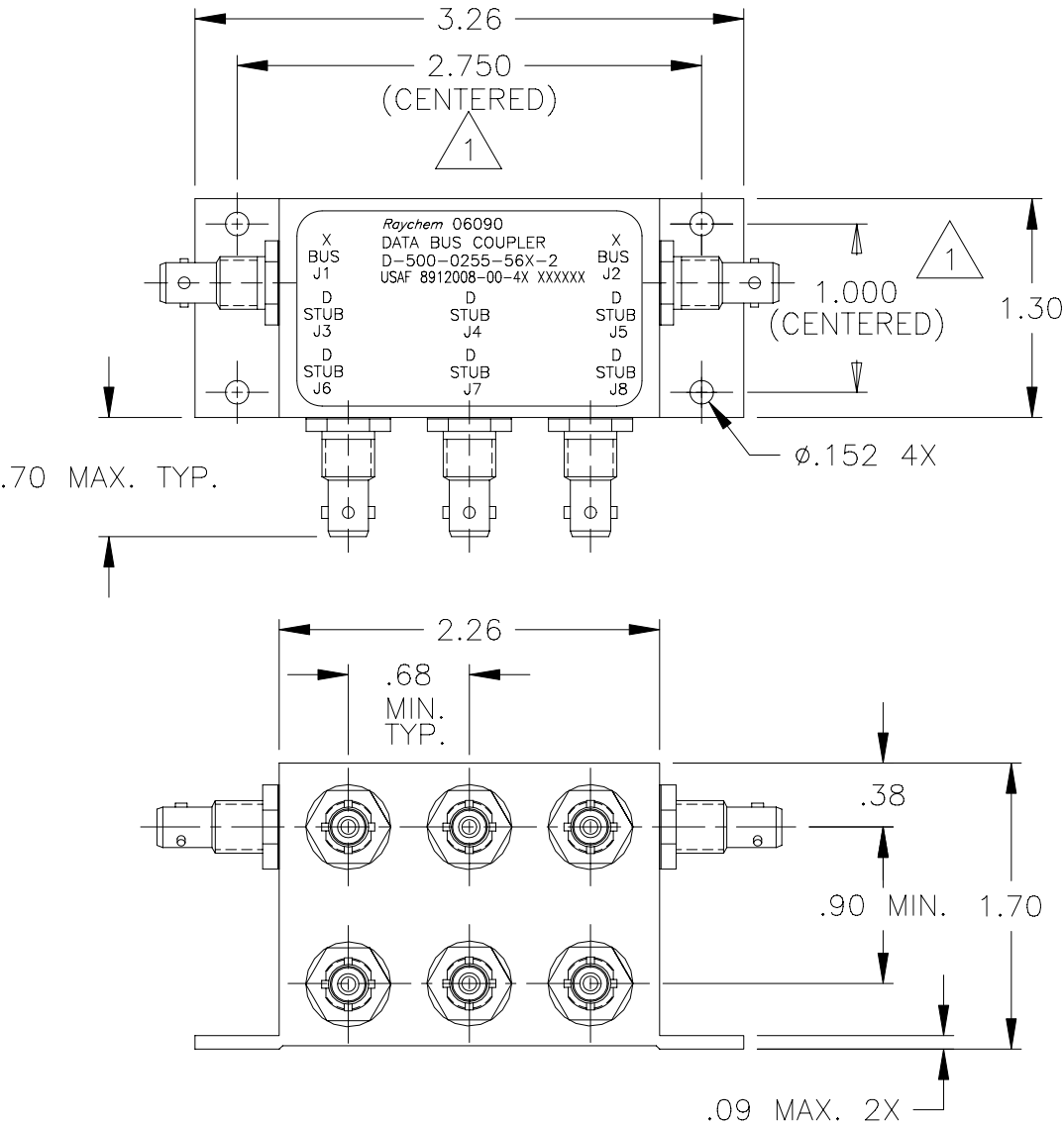
SIDE MOUNT BUS CONFIGURATION
