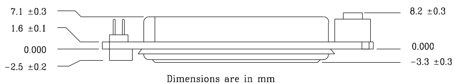
Figure 4-3. Mechanical Dimensions - Side View
