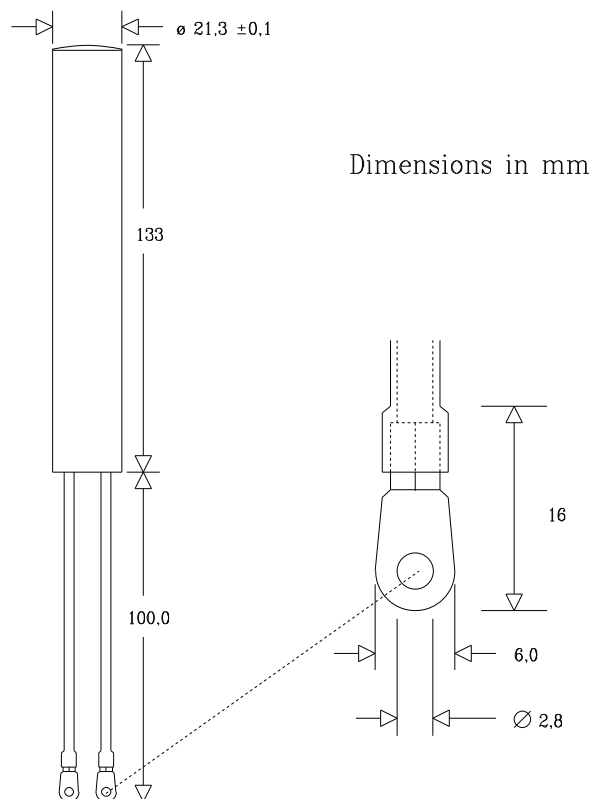
Figure 5-7. Stick Antenna RI-ANT-P02A
