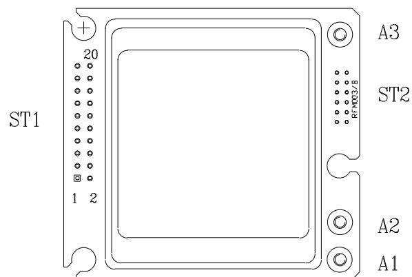
Figure 3-2. Bottom View
